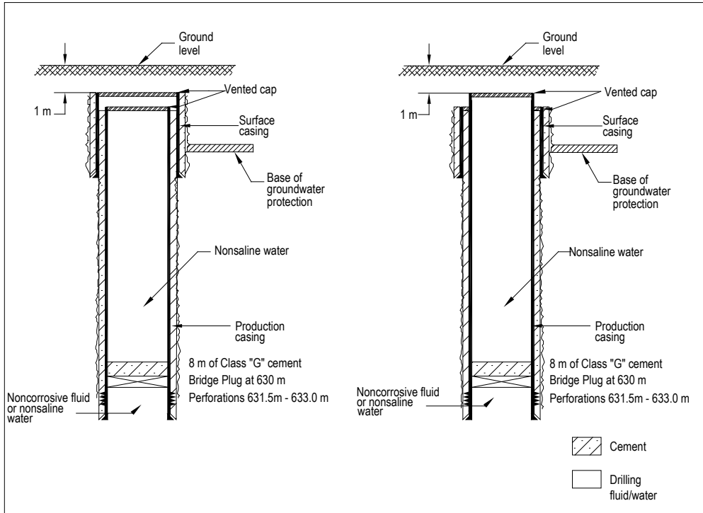
Figure 13. Examples of cased-hole abandonment for non-level-A intervals
