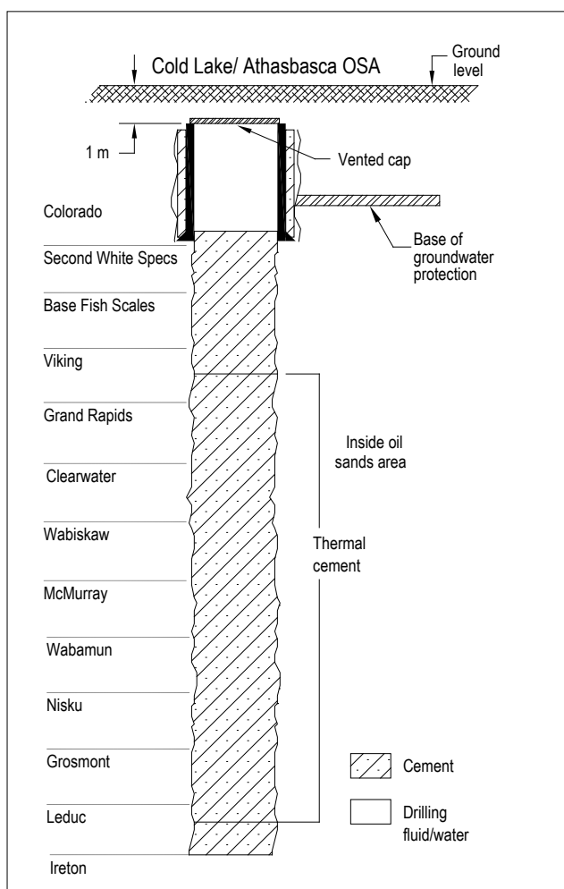
Figure 6. Plug placement example for the Cold Lake and Athabasca oil sands areas
